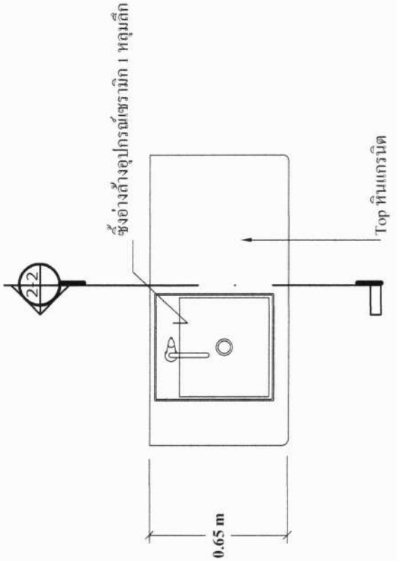
TOP VIEW SCALE 1 : 20
