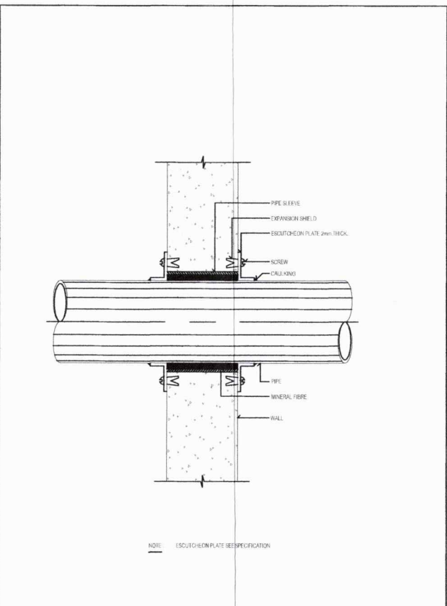
PIPE SLEEVE THROUGH INTERIOR WALL
