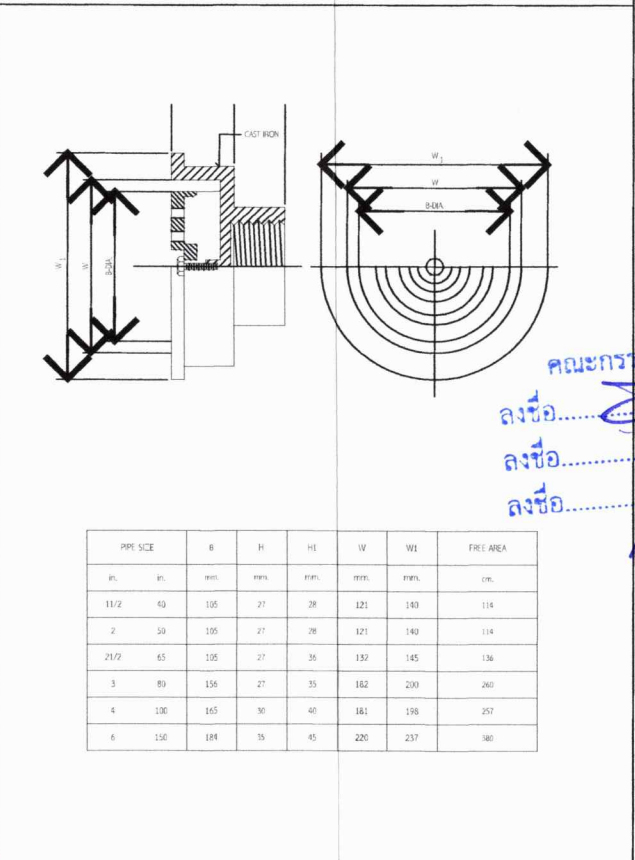
AIR VENT CAP (VTA WALL TYPE)
