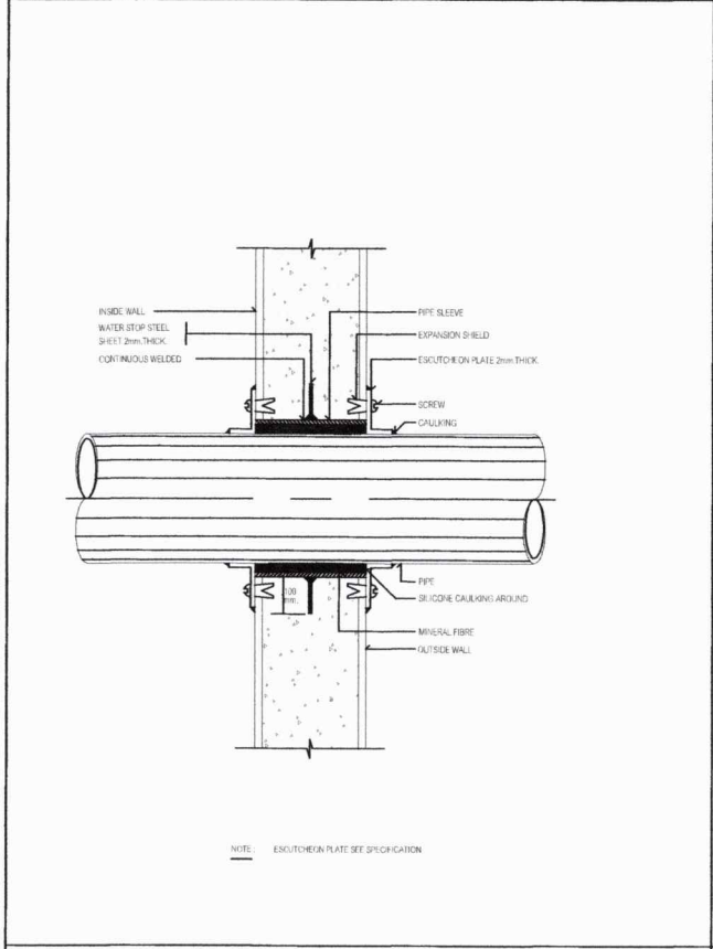
PIPE SLEEVE THROUGH OUTSIDE WALL
