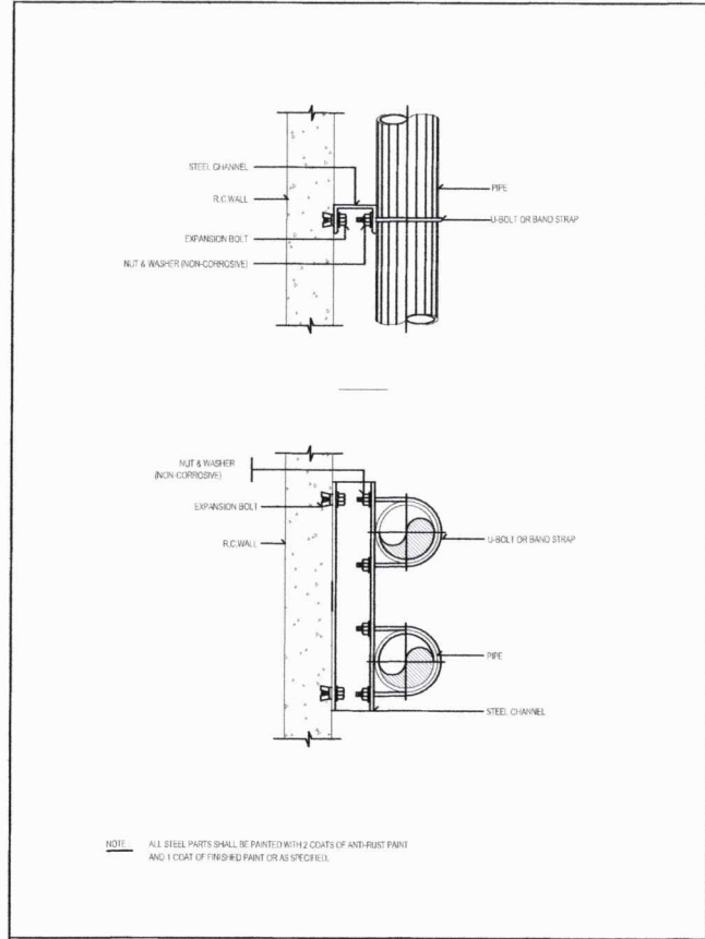
PIPE SUPPORT TO WALL
