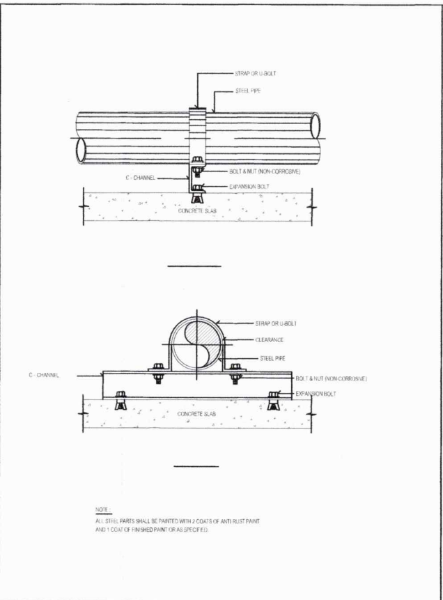
PIPE SUPPORT TO FLOOR
