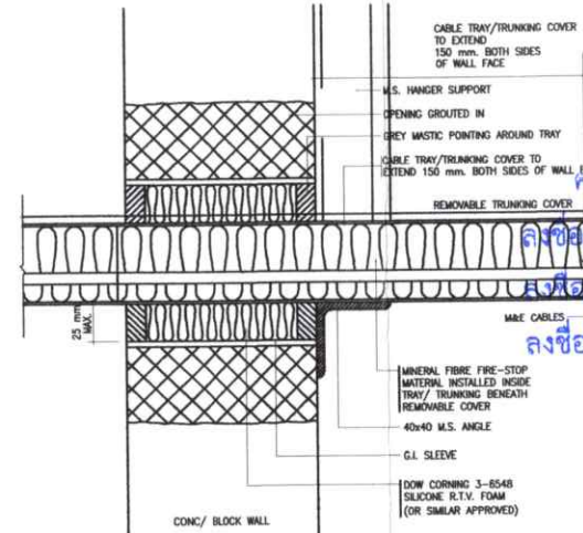
04 DETAIL-FIRE STOP TO CABLE TRAY/ TRUNKING THROUGH WALL N.T.S.
