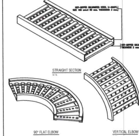
12 DETAIL-CABLE TRAY N.T.S.
