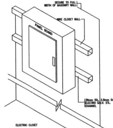
03 DETAIL-PANEL BOARD INSTALLATION ON MASONRY WALL N.T.S.
