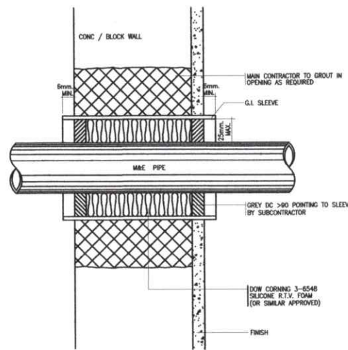
05 DETAIL-SLEEVE THROUGH FIRE WALL-ABOVE CEILING N.T.S.
