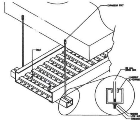
01 DETAIL-CABLE TRAY SUPPORT N.T.S.
