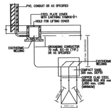
DOWN CONDUCTOR FROM EARTHING PIT TO GROUND ROD
