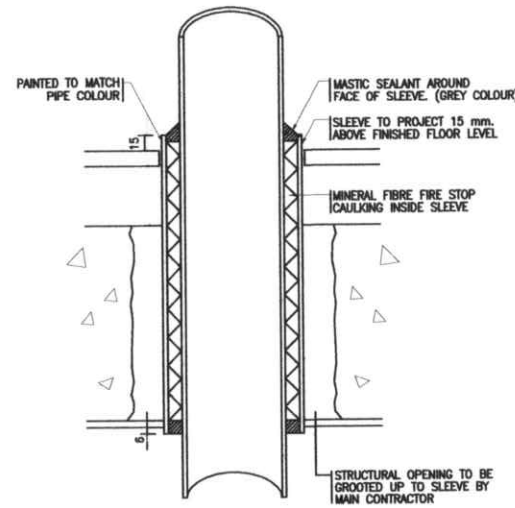
07 DETAIL-FIRE SLEEVE THROUGH FLOOR SLAB N.T.S.
