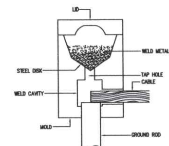
DETAIL FOR EXOTHERMIC WELDING
