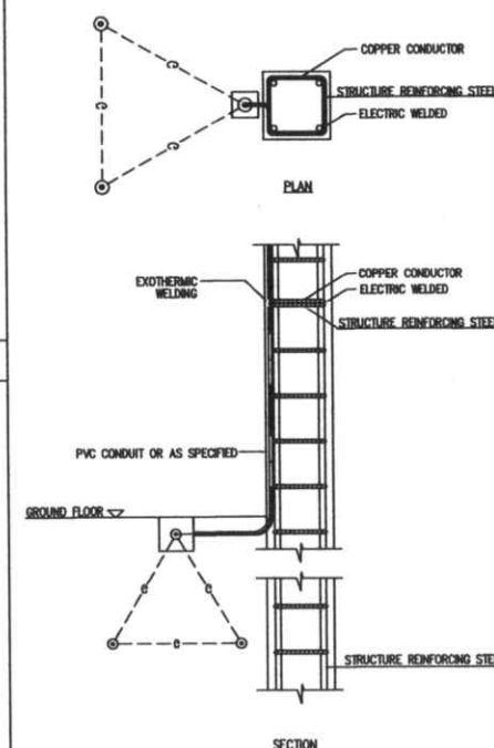
DOWN CONDUCTOR FROM EARTHING PIT TO GROUND ROD
