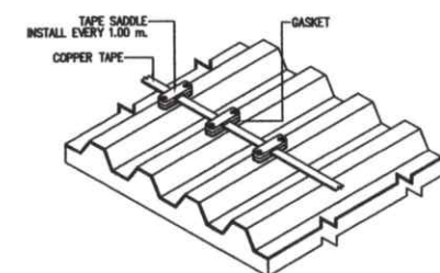
COPPER TAPE FITTING
