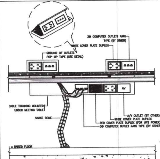
08 DETAIL OF OUTLETS INSTALLATION FOR MEETING TABLE N.T.S.
