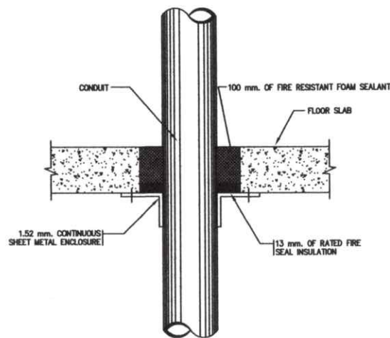
09 DETAIL-CONDUIT FLOOR PENETRATION N.T.S.
