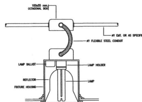
03 RECESSED MOUNTED DOWNLIGHT N.T.S.
